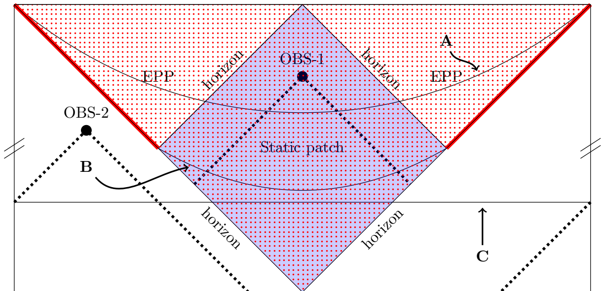
Figure 2: Penrose diagram for the de Sitter space. The blue shaded part – the static patch(SP), the part with red dots – expanding Poincaré patch(EPP). A line is the Cauchy surface for the field in EPP, B line is the Cauchy surface for the field in SP, C line is the Cauchy surface for the field in the global de Sitter space. Note that if we consider the Cauchy surface in the SP as the Cauchy surface in the EPP, then there are the zones where it becomes light-like – thick red lines. OBS-1 is the observer inside the static patch, while OBS-2 is the observer outside the static patch. Dashed black lines represent the boundary of the causal past for the observers.
