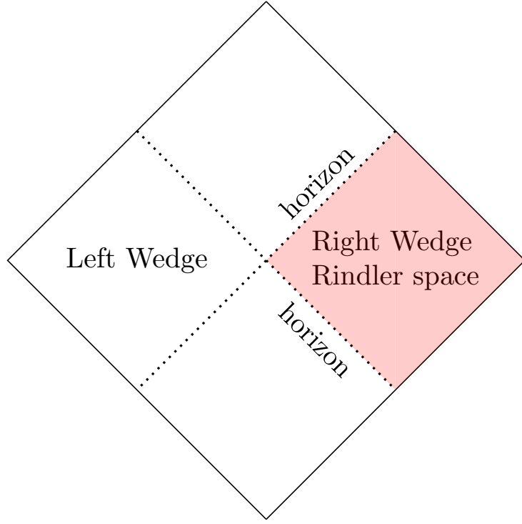
Figure 3: Penrose diagram of the Rindler space. The Rindler space is bordered by a Killing horizon.
