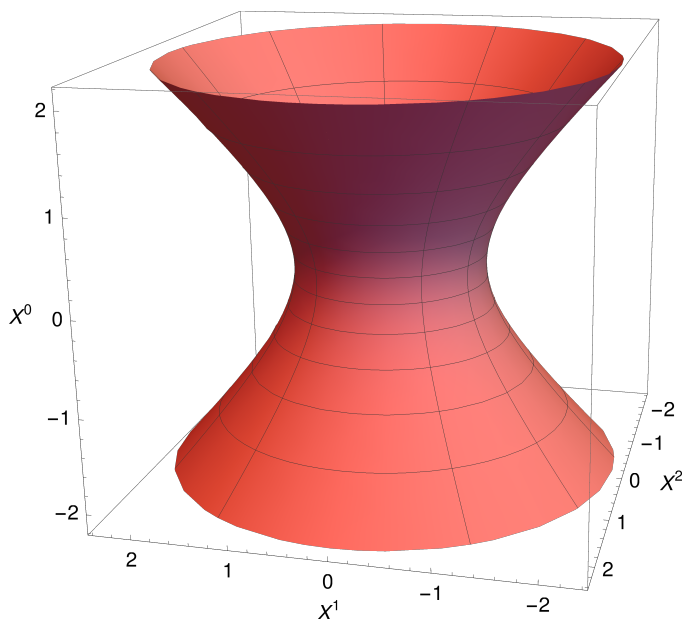
Figure 1: The de Sitter space with unit radius embedded in the three dimensional ambient Minkowski space.
